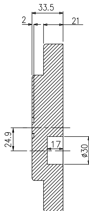
SECTION – FF
